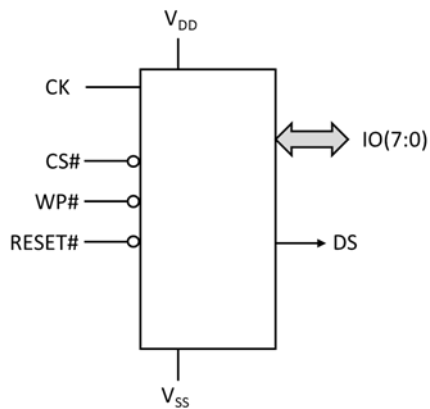
OSPI, QSPI, DSPI, xSPI (24-PIN BGA)
