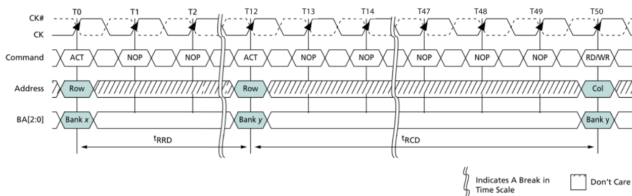
Figure 4 – ACTIVE Command Example: Meeting t_{RRD} (MIN) and t_{RCD} (MIN)
