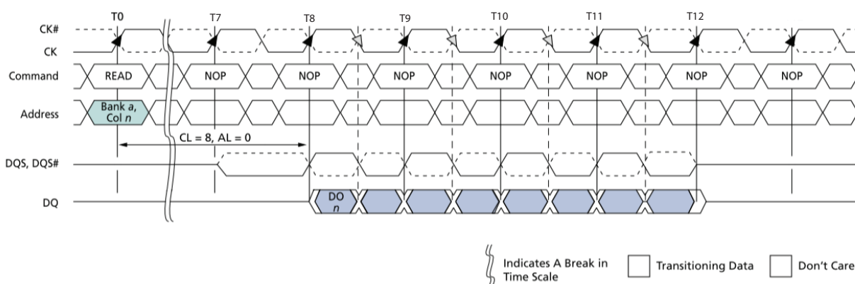
Figure 6 – READ Command Timing
