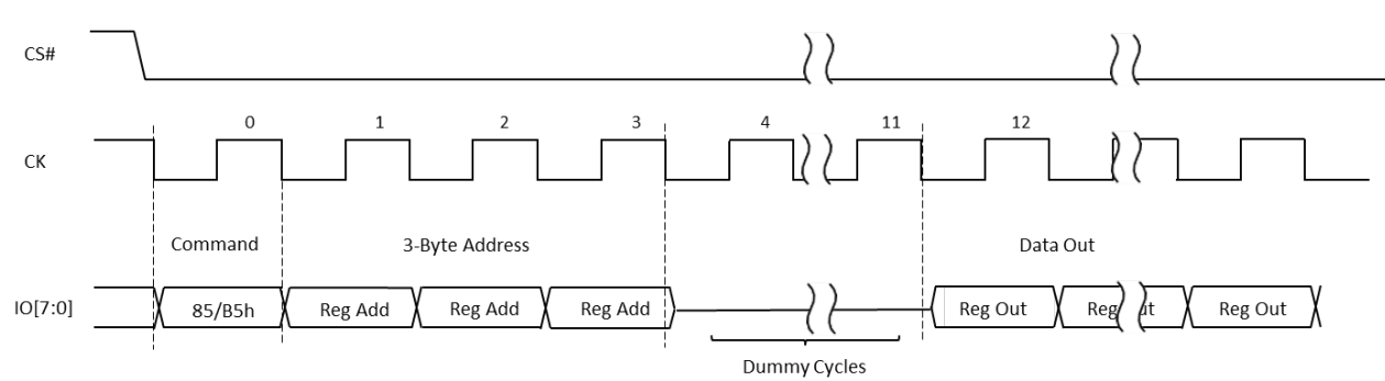
Figure 6: Read Nonvolatile/Volatile Register
